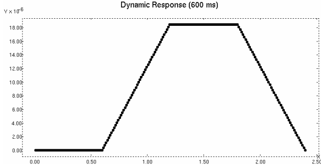
Figure 5: Slow Switch Response (600ms Rise Time)
