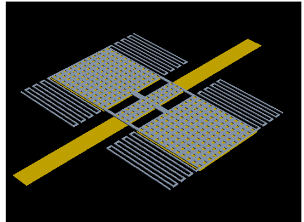
Figure 2: 3-D Rendering of RF MEMS Device
