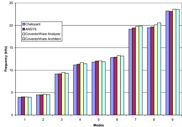
Figure 4: Modal Response of Four Meander Spring
