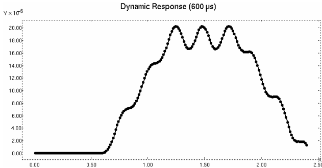
Figure 6: Fast Switch Response ( 600\mu\text{s} Rise Time)
