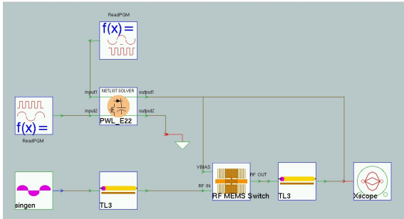
Figure 7: Chatoyant Schematic of Full System Simulation
